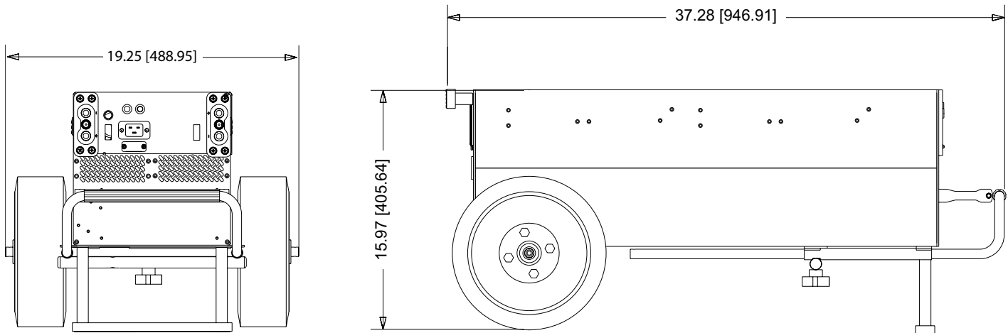
Figure 2.5.1 – TI3560 12-24 GPU physical dimensions
