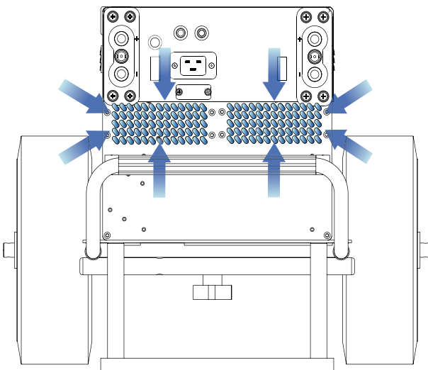
Figure 2.7.3: Front Inlet
