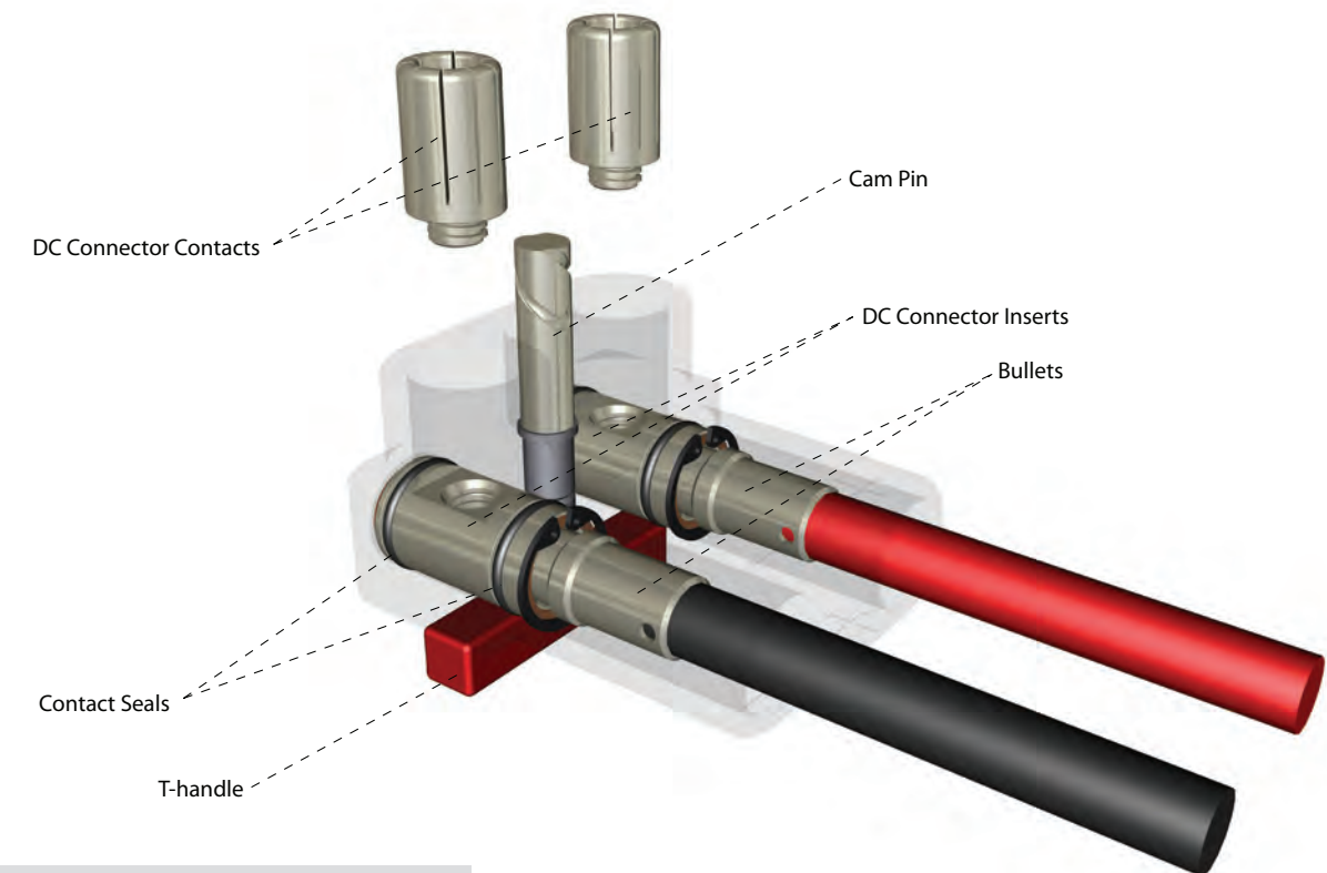
Figure 4: Cable Crimp Bullets: TI2005-199
